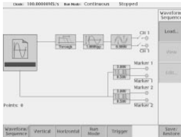
Figure 2-31: Initial screen
