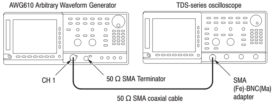
Figure 2-30: Cable connection between AWG610 Arbitrary Waveform Generator and digital storage oscilloscope
