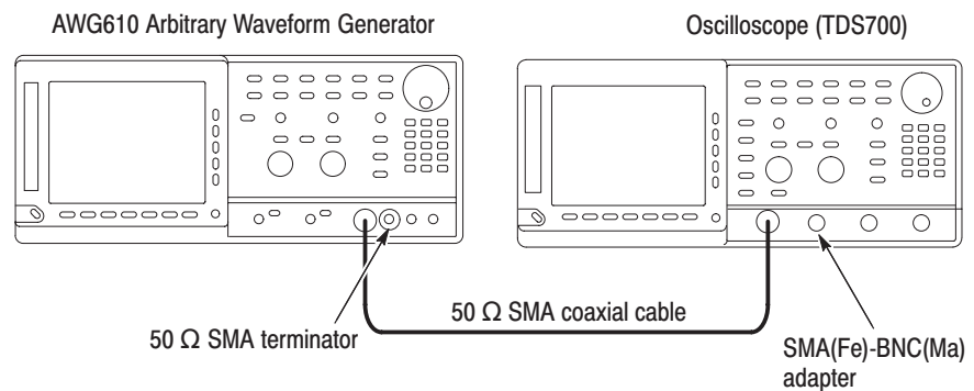
Figure B-27: Marker output initial test hookup
