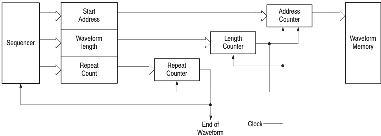
Figure 2-29: Relationship between memory address control and waveform memory
