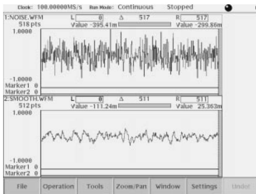
Figure 3-64: Noise waveforms before (upper) and after (lower) 7-point smoothing
