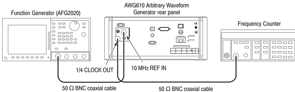
Figure B-24: 1/4 Clock frequency and 10 MHz reference input initial test hookup
