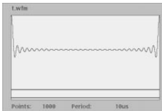
Figure 3–59: Waveform generated by the Example 2 equation
