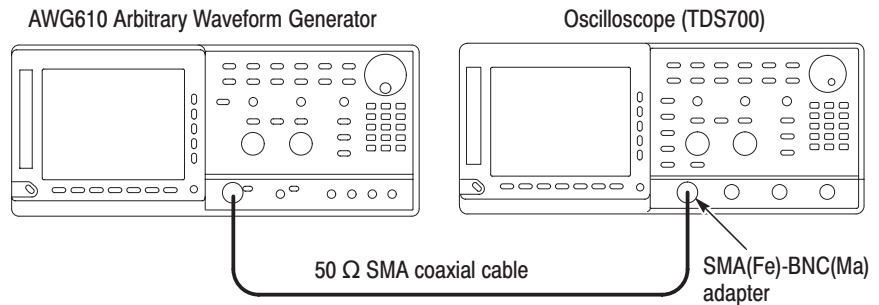
Figure B-16: Event input and enhanced mode initial test hookup
