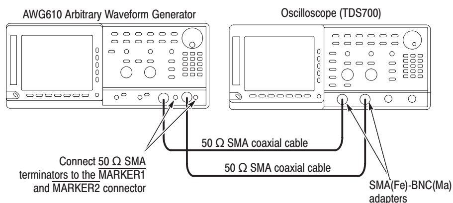
Figure B-28: Marker delay test hookup
