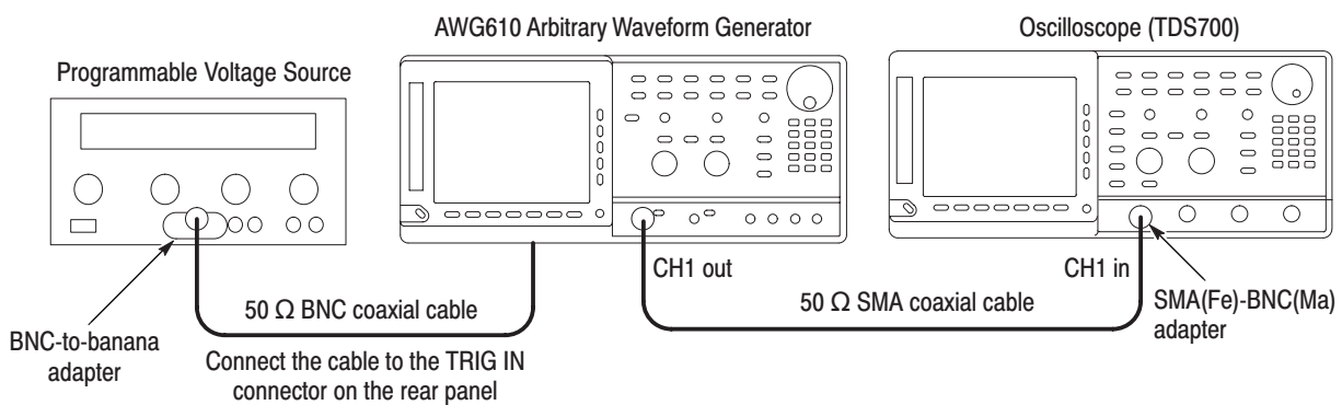
Figure B-15: Trigger input initial test hookup
