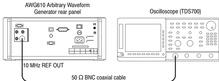
Figure B-26: 10MHz Reference output level initial test hookup
