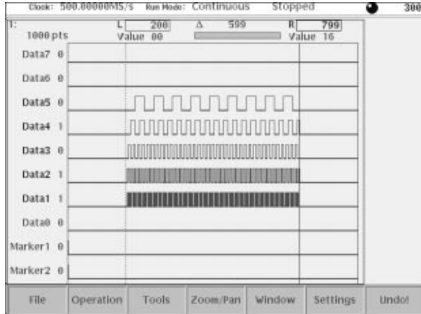
Figure 3-17: Area cursors
