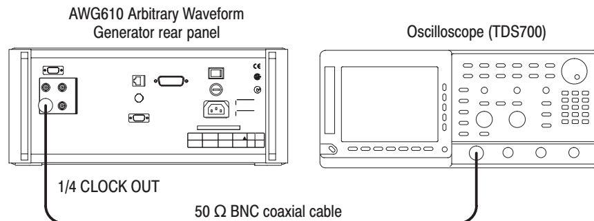
Figure B-25: 1/4 Clock output level initial test hookup
