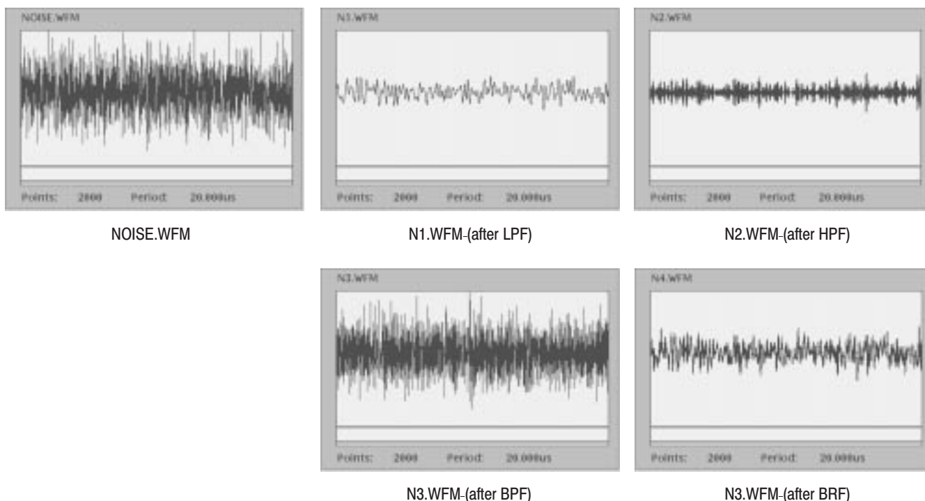
Figure 3-63: Noise waveforms after filtering
